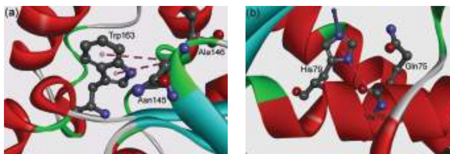
Fig. 7. Example of the structure preferred amide- \pi interactions of FeSOD from the Thermosynechococcus elongatus (PDB code 1my6): a) parallel-displaced and b) T-shaped structure. The interactions are marked with dashed lines.
