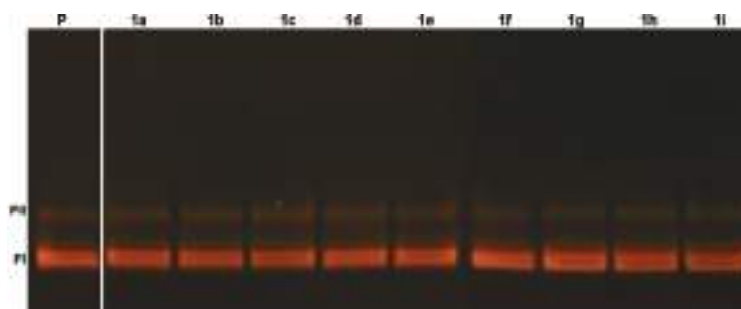
Fig. 7. Agarose gel electrophoretic analysis of plasmid pUC19 without (P) and with derivatives 1a–i (1 mM).
