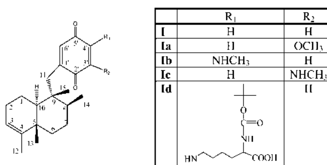
Chart 1. Structures of Quinones
