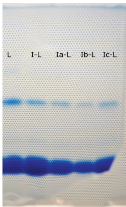
Figure 1. SDS electrophoregram.
