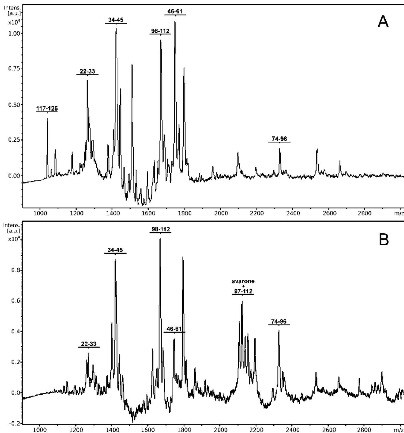
Figure 4. MALDI TOF mass spectra after tryptic digestion of nonmodified lysozyme (A) and lysozyme–avarone conjugate (B).
