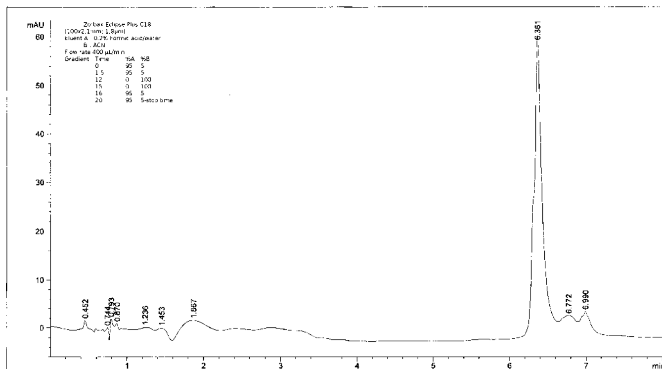
Figure 2. HPLC chromatogram of the avarone–lysozyme conjugate.
