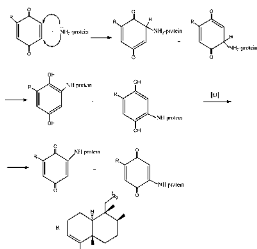
Scheme 1. Mechanism of Protein Amino Group Modification by Avarone
