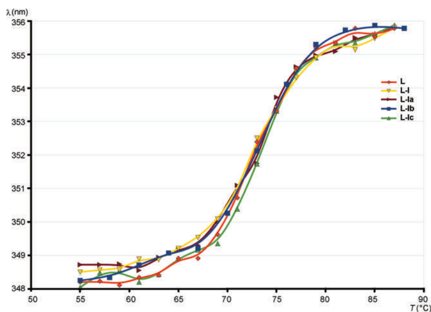
Figure 6. Change of fluorescence wavelength maximum with temperature.
