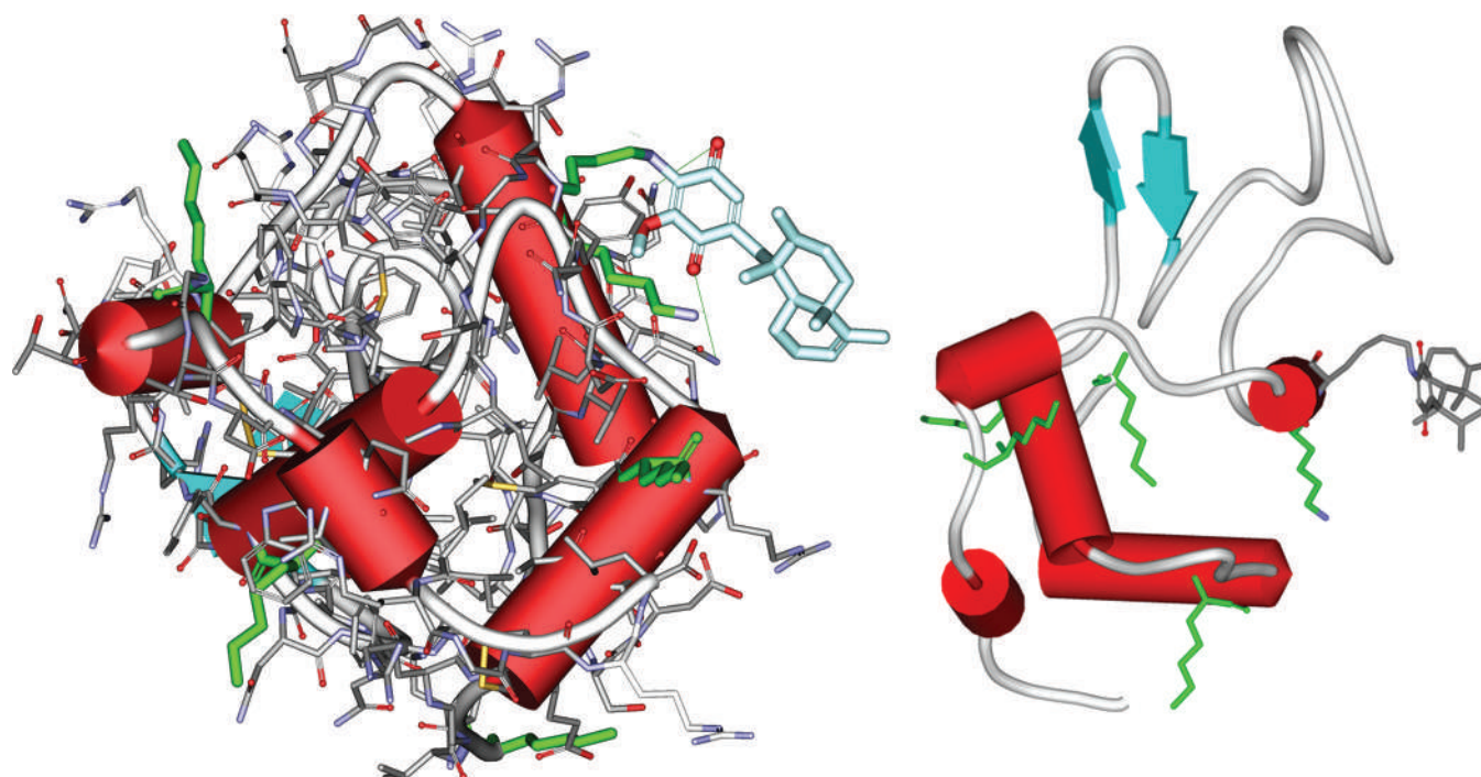
Figure 5. Images of lysozyme conjugate with avarone bound to lysine 97.
