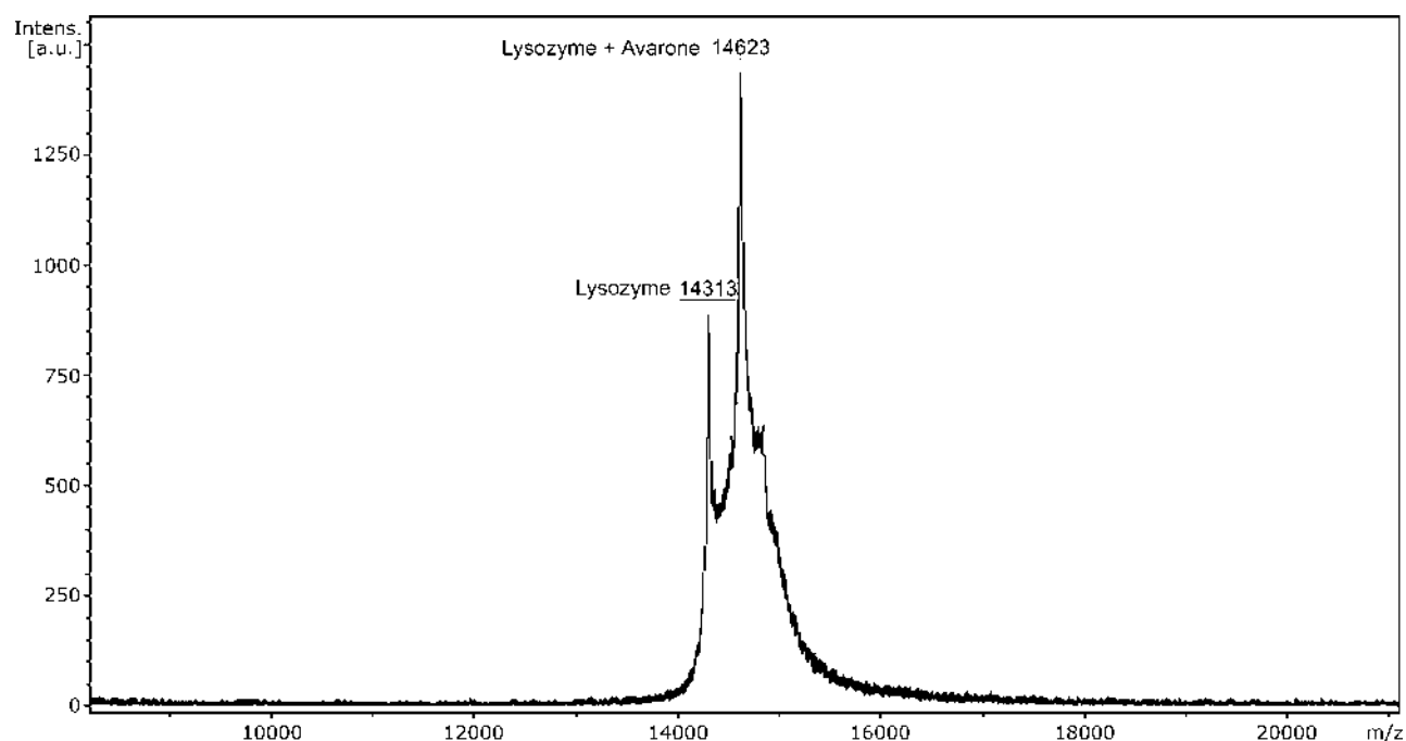
Figure 3. MALDI TOF mass spectrum of lysozyme and its conjugate with avarone.
