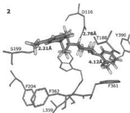
Fig. 3. Ligand 2 docked in the active site
