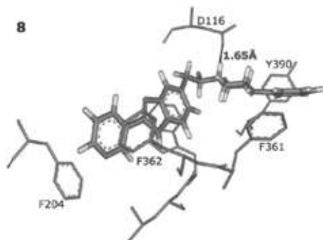
Fig. 9. Ligand 8 docked in the active site.
