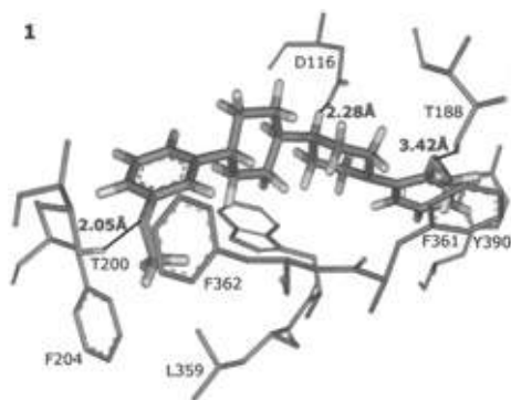
Fig. 2. Ligand 1 docked in the active site.
