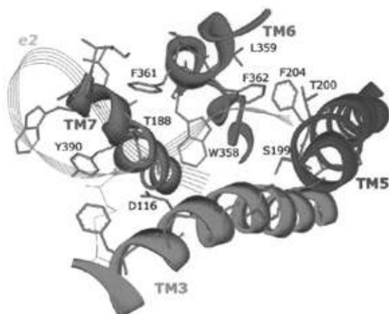
Fig. 1. The binding site of the 5-HT 1A receptor model.
