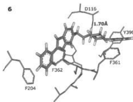
Fig. 7. Ligand 6 docked in the active site.
