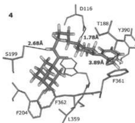
Fig. 5. Ligand 4 docked in the active site
