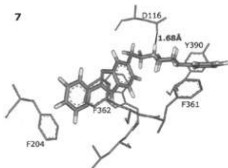
Fig. 8. Ligand 7 docked in the active site.
