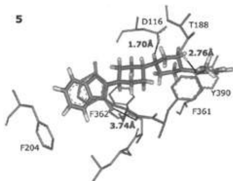
Fig. 6. Ligand 5 docked in the active site
