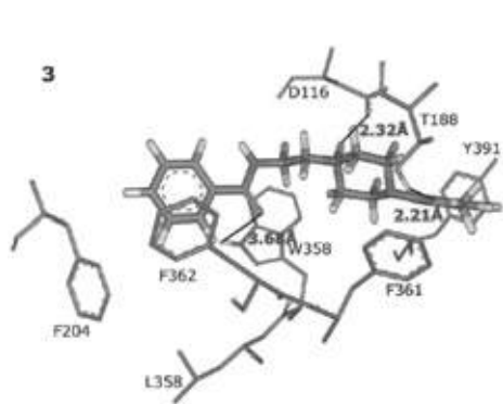
Fig. 4. Ligand 3 docked in the active site
