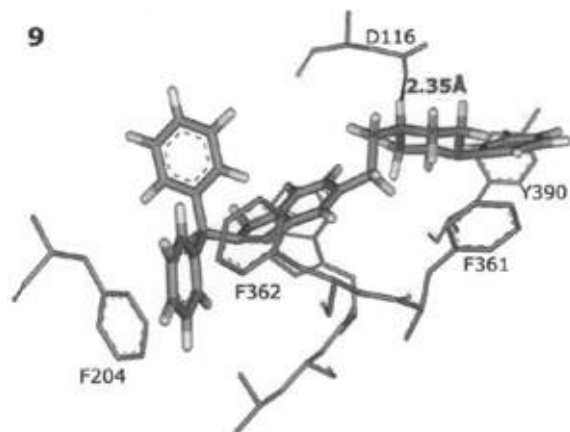
Fig. 10. Ligand 9 docked in the active site.
